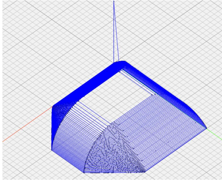
Figure 4: G-Code figure of the new test shape, view #4
