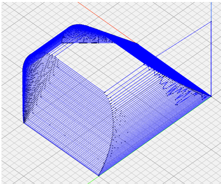
Figure 1: G-Code figure of the new test shape, view #1
