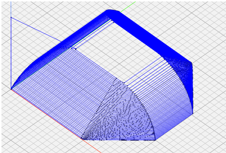
Figure 3: G-Code figure of the new test shape, view #3
